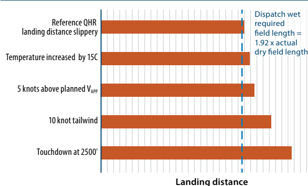
Figure 12. Wet landing distance – BA: Medium
