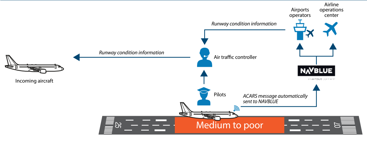
Figure 2. Example automatic braking action data collection and transmission process
