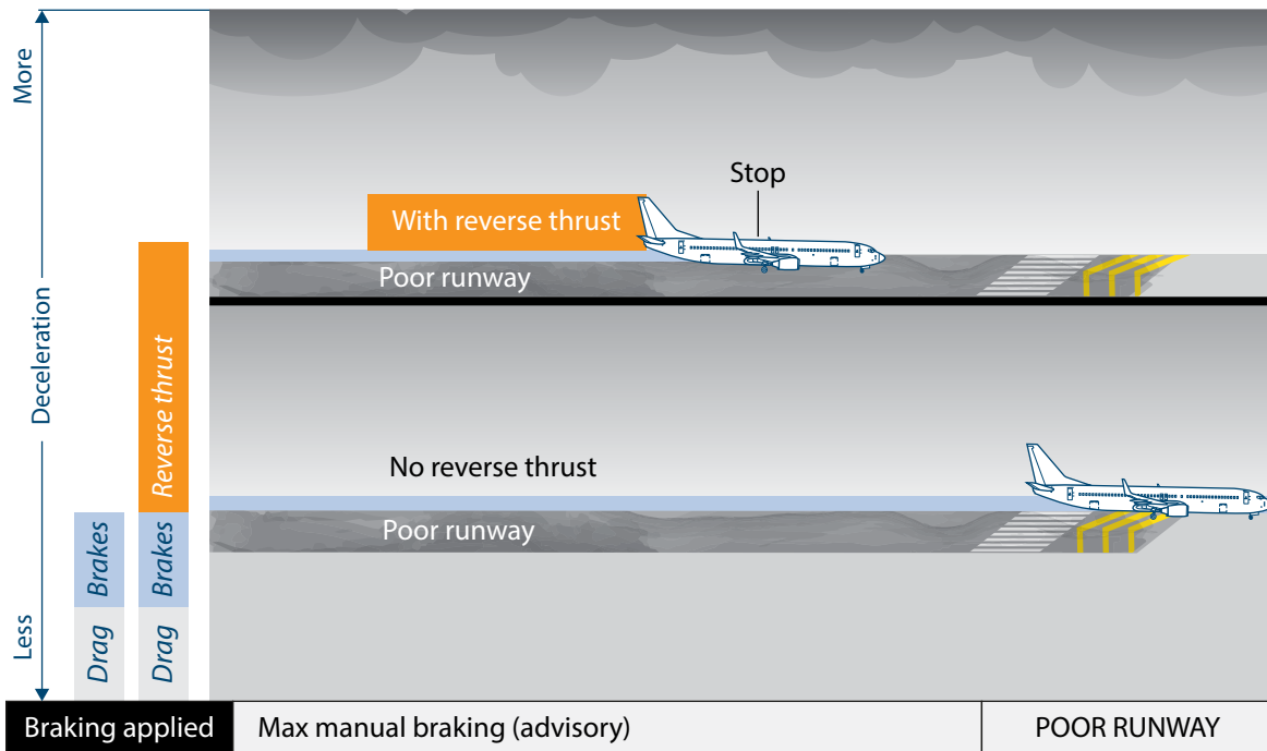
Figure 14. Additive thrust reversers
