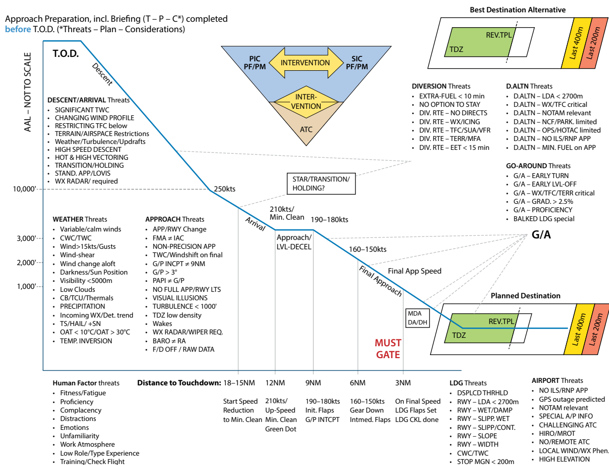
Figure 10. Example safe arrival planning (based on medium to large turbofan aircraft (e.g., A320/B737), adaption for different aircraft type may be needed)
