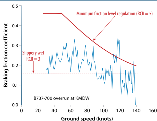
Figure 19. Example of low braking friction on a wet grooved runway
