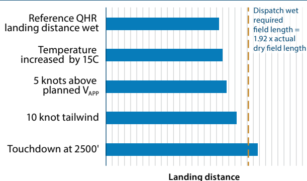
Figure 11. Wet landing distance – BA: Good
