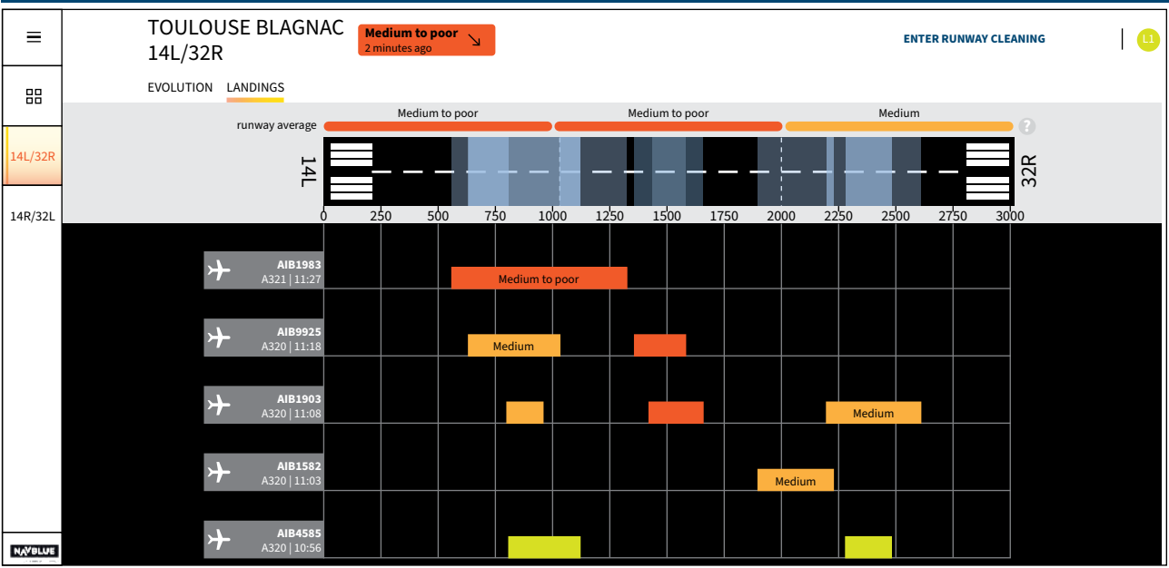
Figure 3. Example of braking action data monitoring
